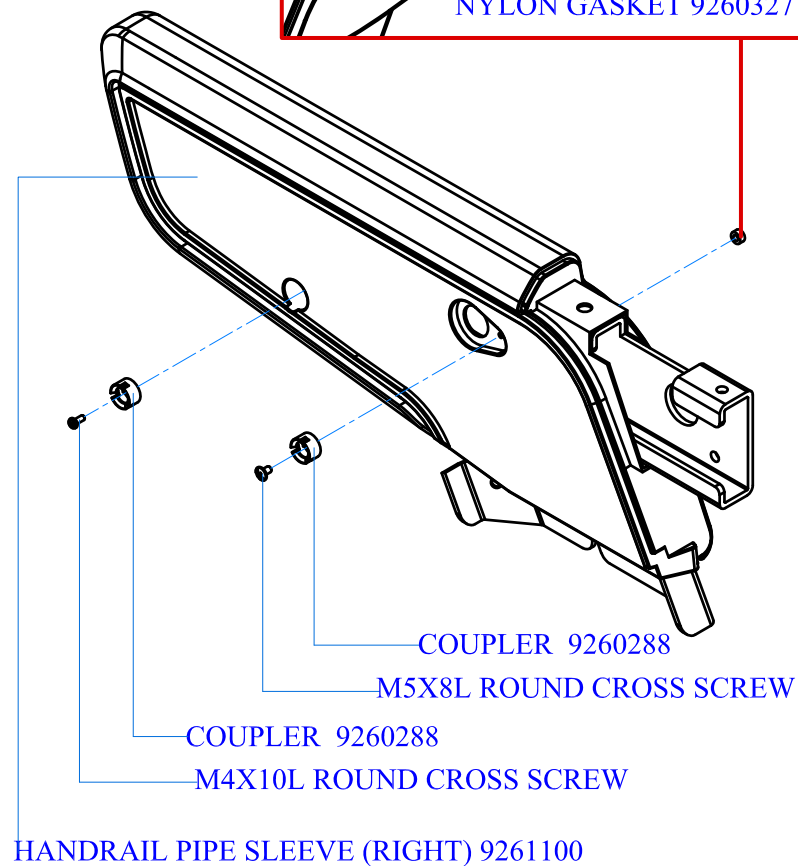
NYLON GASKET 9260327
