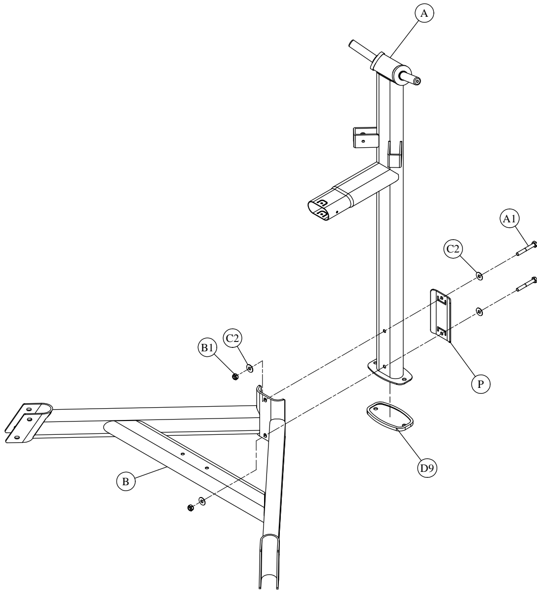
Above shows STEP 1 assembled and completed
