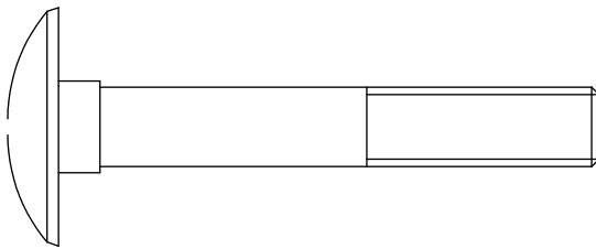
A4.M10X65L SQUARE NECK CARRIAGE SCREW .....2PCS
