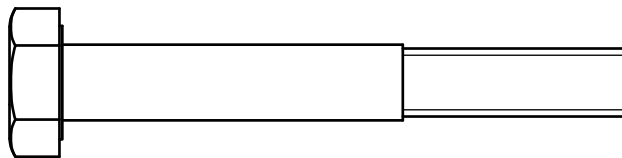
A5.M10X70L HEX HEAD SCREW.....[4PCS]
