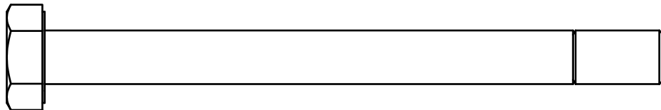
(A12)HEX BOLT M10X115L PARTIAL THREAD QTY.3
