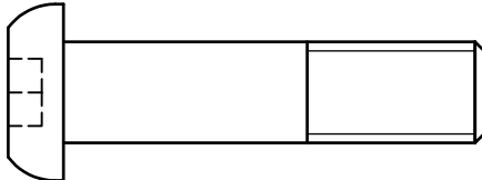
(A14)ROUND ALLEN HEAD M12X50L PARTIAL THREAD QTY.8
