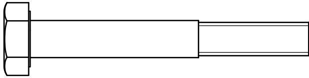
(A11)HEX BOLT M10X75L PARTIAL THREAD QTY.2
