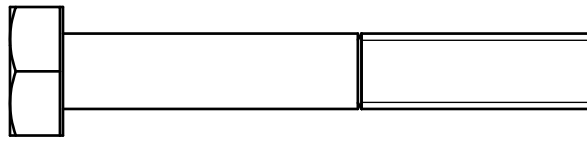
(A22)HEX BOLT M10X70L PARTIALTHREAD QTY.1
