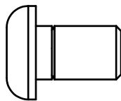
(A13)ROUND INNER SCREW M10X16L PARTIALTHREAD QTY.2
