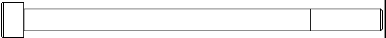
(A19)ROUND INNER SCREW M10X160L PARTIALTHREAD QTY.1
