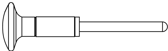
(A19)ROUND INNER SCREW M10X160L PARTIALTHREAD QTY.1
