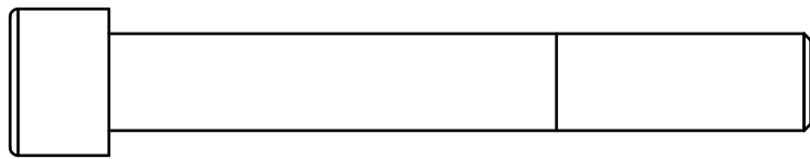
(A17)ROUND INNER HEX M12X85L PARTIALTHREAD QTY.1
