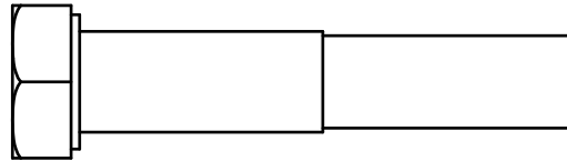
(A16)HEX BOLT M12X60L PARTIALTHREAD QTY.1
