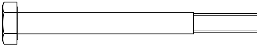
A2.HEX BOLT M10X105L PARTIAL THREAD QTY.2
