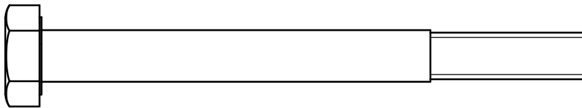
A2.HEX BOLT M10X105L PARTIAL THREAD QTY.2
