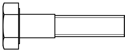
A4.HEX BOLT M10X45L PARTIAL THREAD QTY.7
