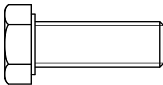
A4.HEX BOLT M10X45L PARTIAL THREAD QTY.7
