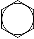
A3. HEX BOLT M10X45L PARTIAL THREAD QTY.7
