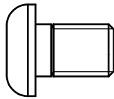
A16.ROUND ALLEN HEAD M10X15L PARTIAL THREAD QTY.6 (pre-installed)
