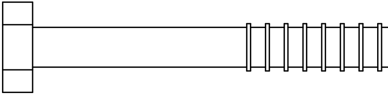
(A1)HEX BOLT 1/2"x3-3/4"L PARTIAL THREAD QTY.4
