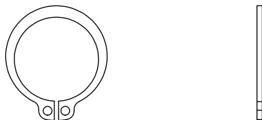
C11.GB893.1-40(Ø40 R Shape) Hole Spring Washer Qty.2(Pre-installed)
