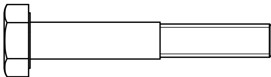
(A3)HEX HEAD BOLT M10X65L PARTIAL THREAD QTY.2
