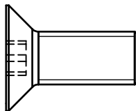
(A4)SOCKER FLAT HEAD SCREW M10X25L PARTIAL THREAD QTY.4
