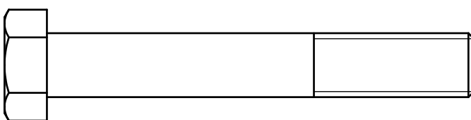
(A5)HEX HEAD BOLT M12X80L PARTIAL THREAD QTY.2
