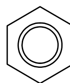
(A5)HEX HEAD BOLT M12X80L PARTIAL THREAD QTY.2
