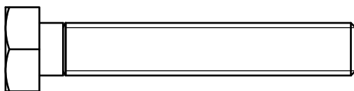
(A4)HEX BOLT M10X60L PARTIAL QTY.4
