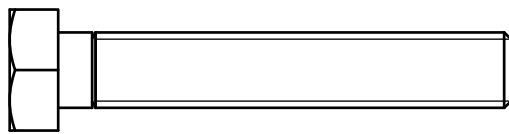
(A3)HEX BOLT M10X60L PARTIAL QTY.4
