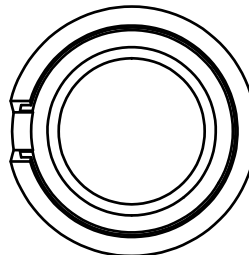
(C6)1/2" BOLT CAP(9212-024) QTY.4
