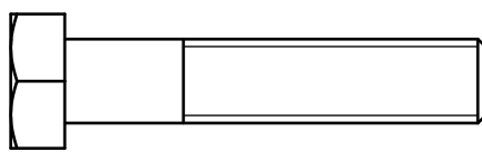
(A4)HEX BOLT M10X50L PARTIAL THREAD QTY.1
