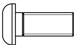
(A5)ROUND ALLEN HEAD M10X25L PARTIAL THREAD QTY.2
