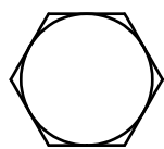
(A4)HEX BOLT M10X50L PARTIAL THREAD QTY.1
