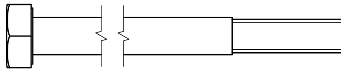
(A3)HEX BOLT M10X120L PARTIAL THREAD QTY.1
