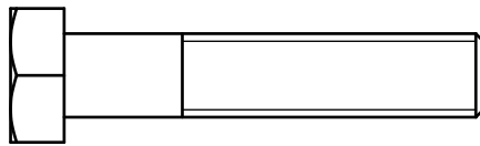
(A4)HEX BOLT M10X50L PARTIAL THREAD QTY.3
