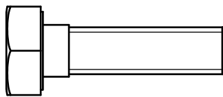
(A5)HEX BOLT M10X35L PARTIAL THREAD QTY.1
