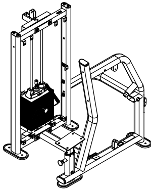
Above shows STEP 4 assembled and completed
