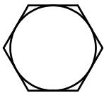
(A4)HEX BOLT M10X50L PARTIAL THREAD QTY.3
