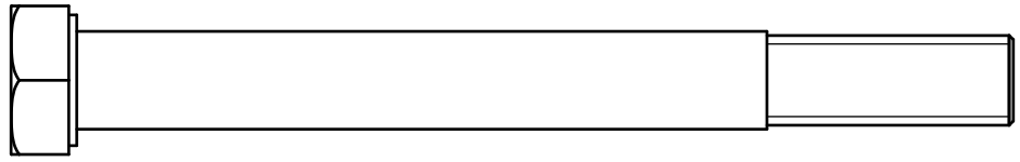
(A1)HEX BOLT M12X115L PARTIAL THREAD QTY.1
