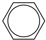
(A5)HEX BOLT M10X35L PARTIAL THREAD QTY.1
