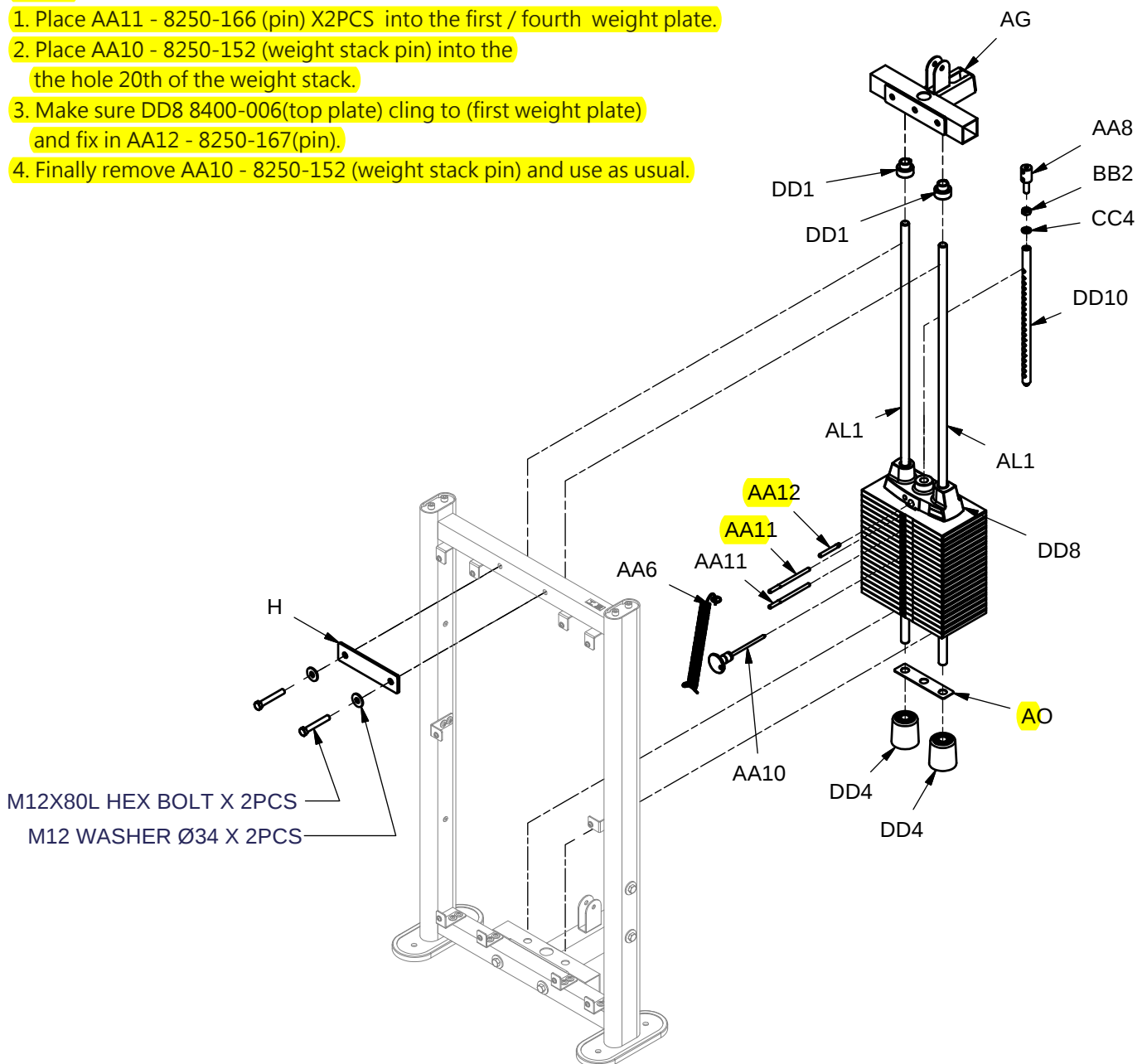
Above shows STEP 4 assembled and completed
