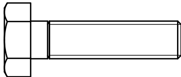
(A2)HEX BOLT M10X40L PARTIAL THREAD QTY.2
