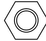
(A1)HEX BOLT M10X50L PARTIAL THREAD QTY.2
