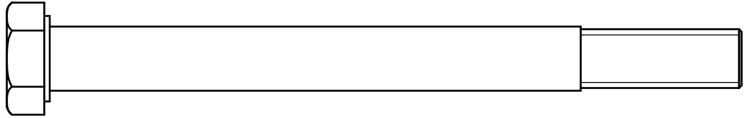
(A2)HEX BOLT M12X130L PARTIAL THREAD QTY.16
