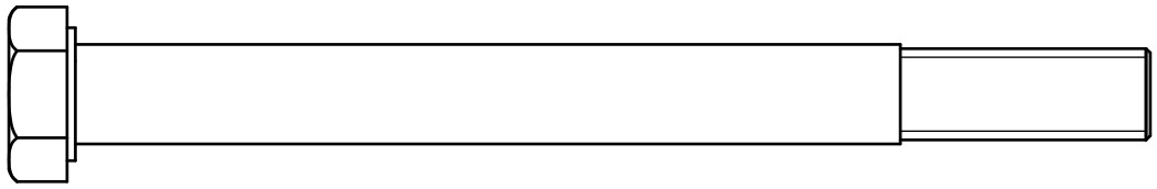
(A1)HEX BOLT M12X130L PARTIAL THREAD QTY.12
