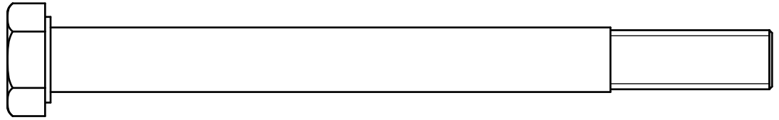
(A2)HEX BOLT M12X135L PARTIAL THREAD QTY.16
