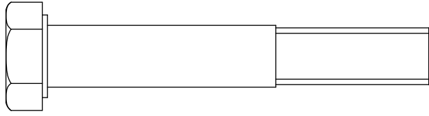
A12.M12X80L Ordinary Hexagonal Head Screw Qty.22
