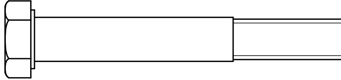
(A2)HEX BOLT M12X85L PARTIAL THREAD QTY.1
