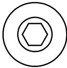
(A4)ROUND INNER HEX SCREW M10X20L PARTIAL THREAD QTY.2
