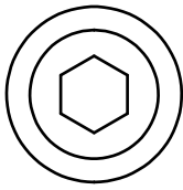
(A1)ROUND INNER HEX SCREW M12X90L PARTIAL THREAD QTY.2
