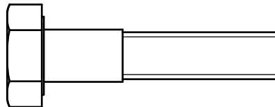
(A5)HEX BOLT M10X50L PARTIAL THREAD QTY.4
