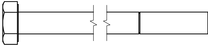
(A3)HEX BOLT M10X135L PARTIAL THREAD QTY.1
