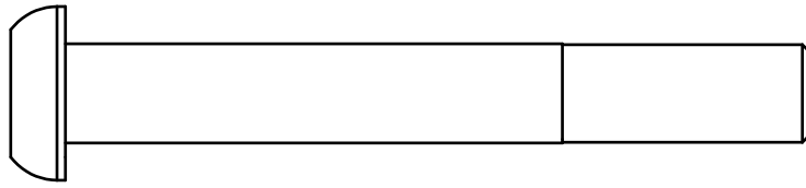
(A1)ROUND INNER HEX SCREW M12X90L PARTIAL THREAD QTY.2
