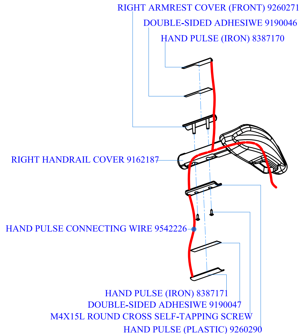
(RIGHT) HANDLE BAR SET 22PB10-11
