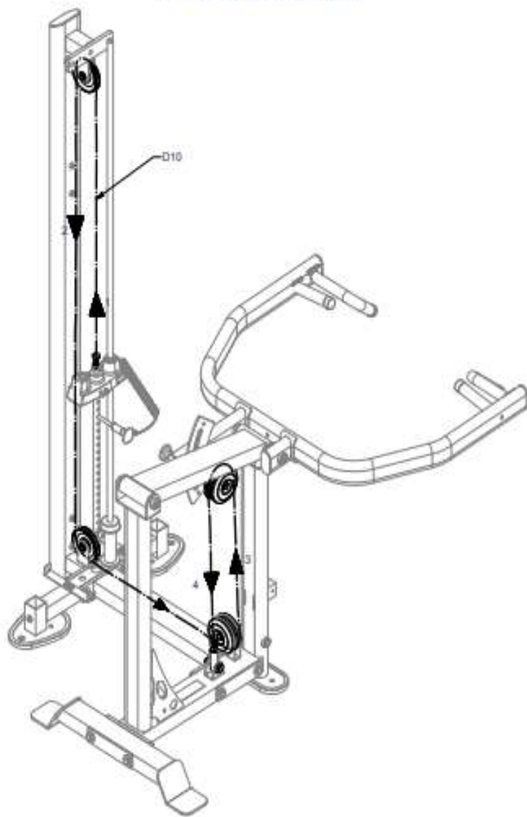
Cable Configuration Diagram
