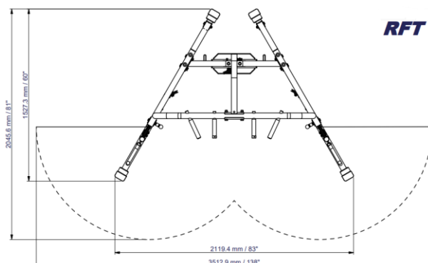
Floor Space Dimensions: L2119.4 x W1527.3 x H2309 mm Live Working Area : L3512.9 x W2045.6 mm
