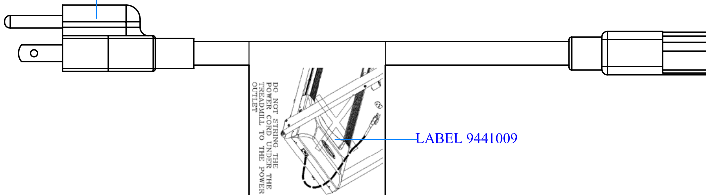
POWER CORD 9541013
