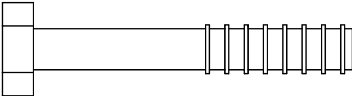
(A2)HEX BOLT 1/2"X3 1/4"L PARTIAL THREAD QTY.10
