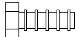
(A6)HEX BOLT 3/8"X1"L PARTIAL THREAD QTY.6
