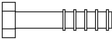
(A7)HEX BOLT 3/8"X1 3/4"L PARTIAL THREAD QTY.15
