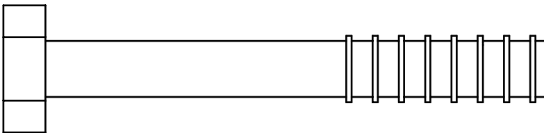
(A3)HEX BOLT 1/2"X3 3/4"L PARTIAL THREAD QTY.2
