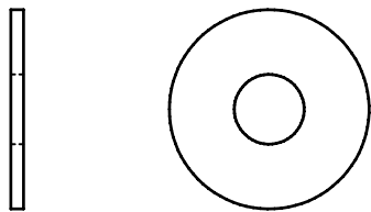
(C10)M8(I.D.)FLAT WASHER Ø24 QTY.2
