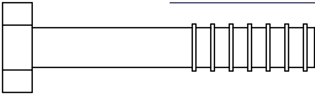
(A1)HEX BOLT 1/2"X3"L PARTIAL THREAD QTY.2
