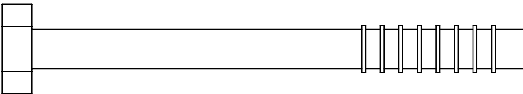
(A5)HEX BOLT 1/2"X5 1/4"L PARTIAL THREAD QTY.1
