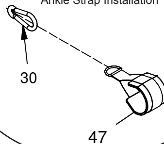
Diagram 2 Ankle Strap Installation
